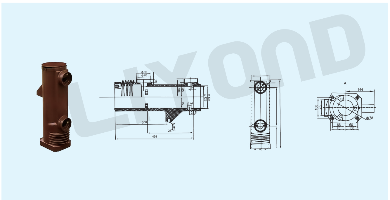
Model No.:LYC163 Name:VS1-12/630-1600A Insulated cylinder
