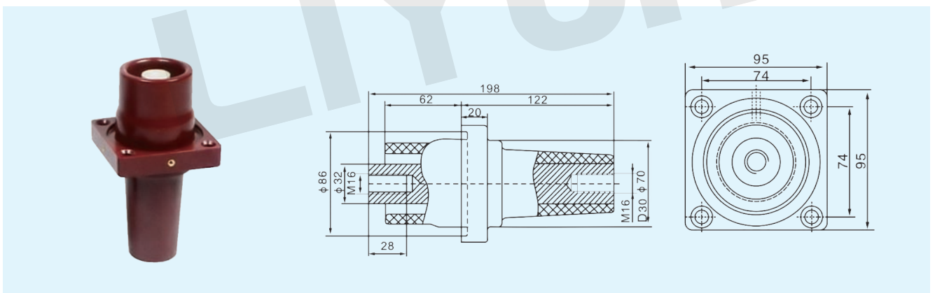
Model No.:LYC169 Name:SF6-24/198 Bushing
