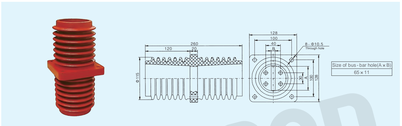
Model No.:LYC143 Name: TG3-12/100x100x260 Bushing
