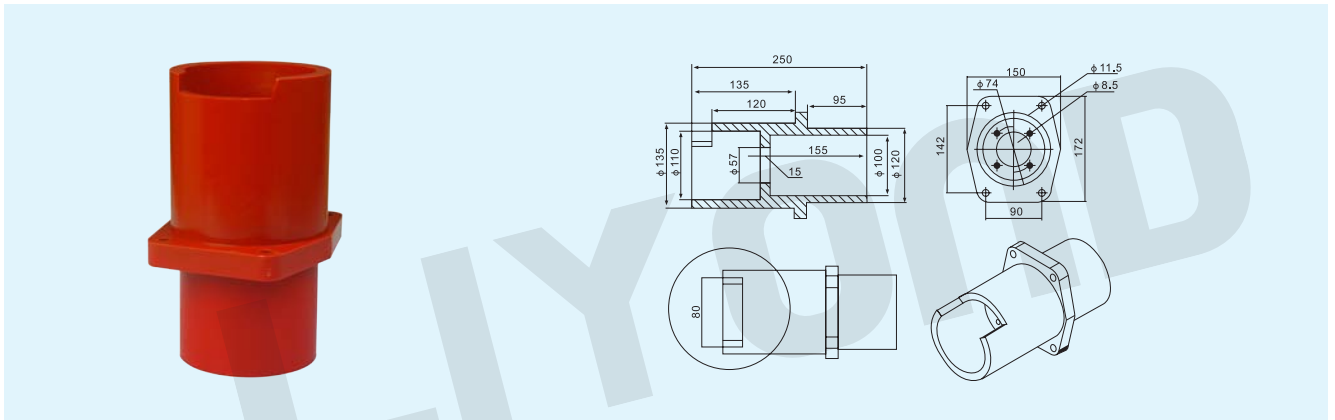
Model No.:LYC142 Name: TG3-12/90x142x250 Bushing
