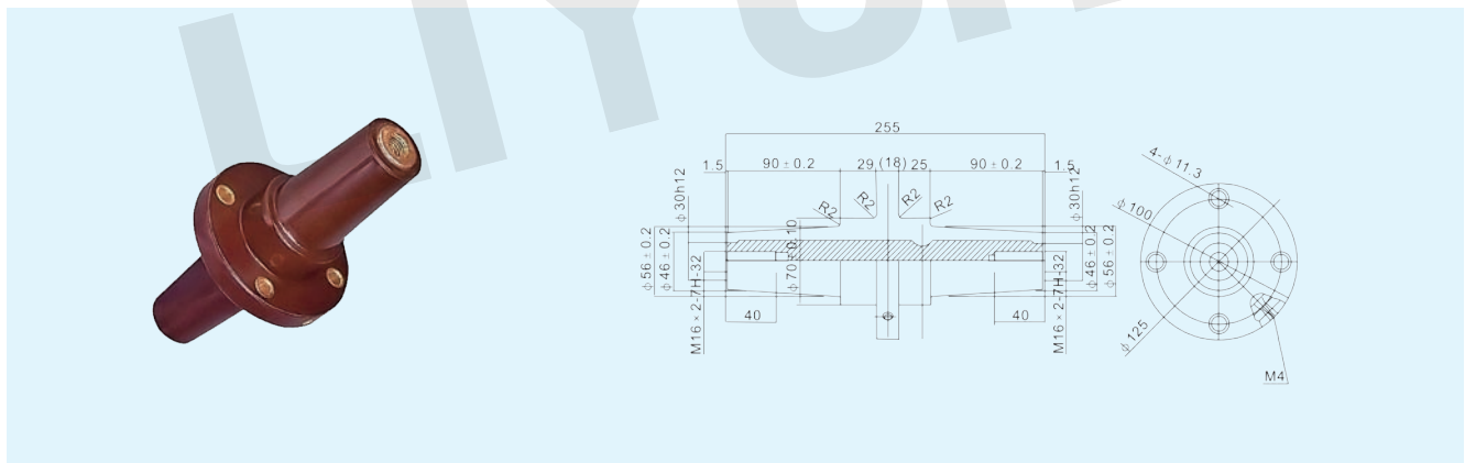
Model No.: LYC166 Name: HCA-12/255 Bushing(European type)
