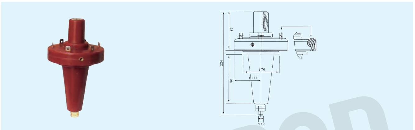
Model No.:LYC168 Name:TGZ-24/224 Bushing(American type)
